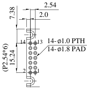
PIN DETAIL
